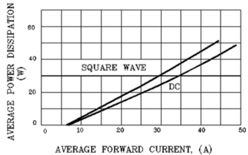
FIG.4. FORWARD POWER DISSIPATION
