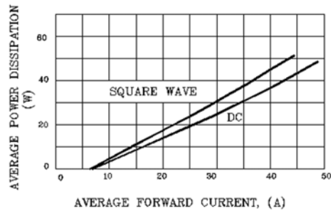
FIG.4. FORWARD POWER DISSIPATION
