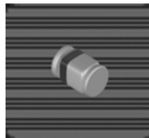
BZM55 Zener Diode Voltage Range: 2.8-75 V Power Dissipation: 500 mW Data Sheet
