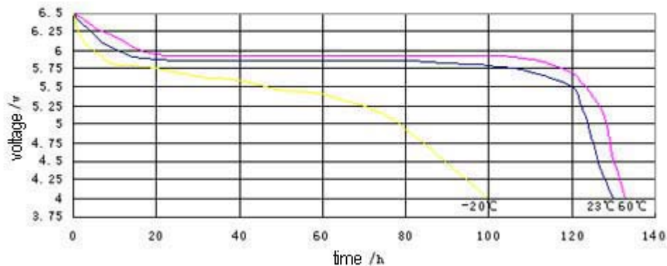
Discharge curve at various temperature(10mA)
