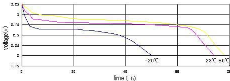
Discharge curve on various temperature (2mA)
