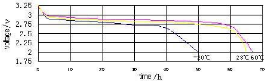
Discharge curve at various temperature(10mA)
