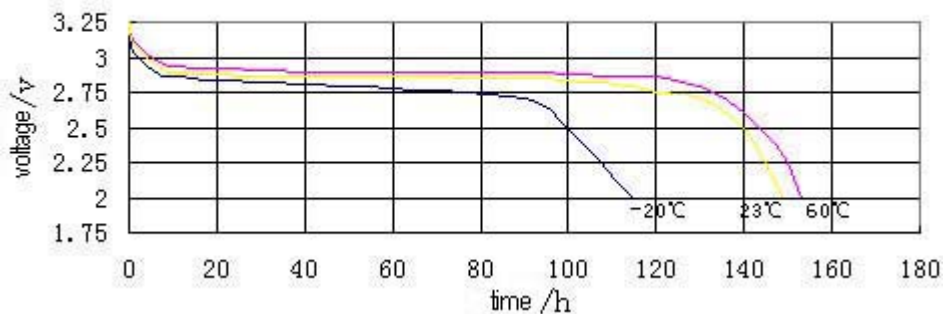
Discharge curve at various temperature (10mA)
