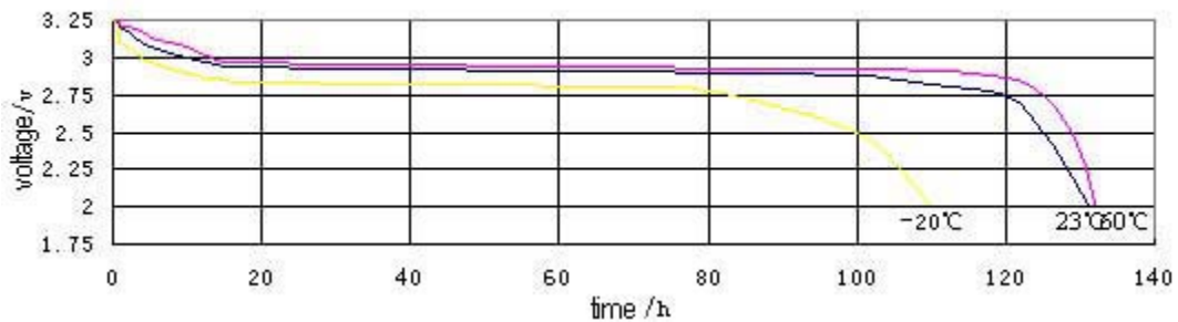
Discharge curve on various temperature (10mA)
