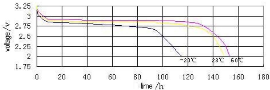
Discharge curve at various temperature (20mA)
