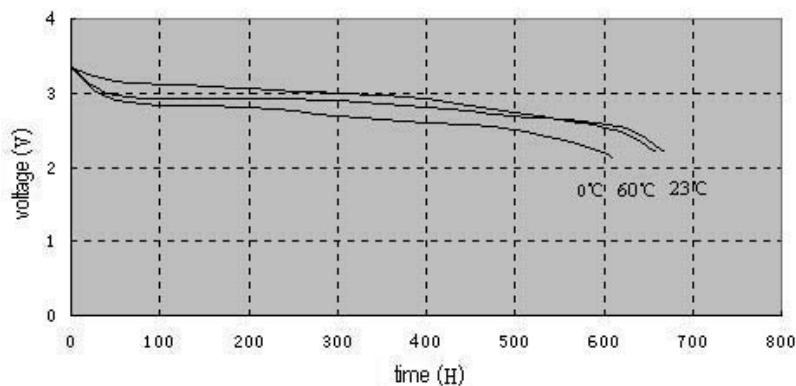
Discharge curve at various temperature (62K Ω)
