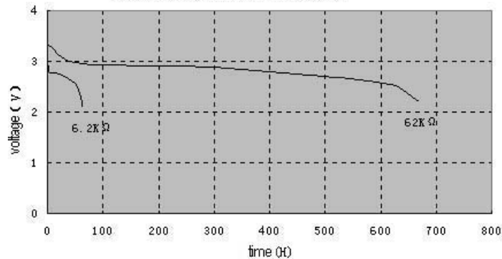
Discharge curve at various load (23°C)
