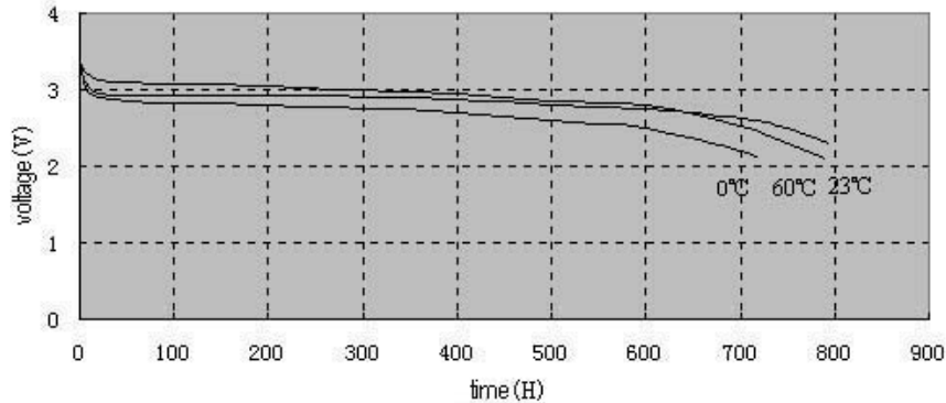
Discharge curve at various temperature(62kΩ)
