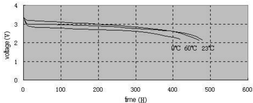
Discharge curve at various temperature (30KΩ)
