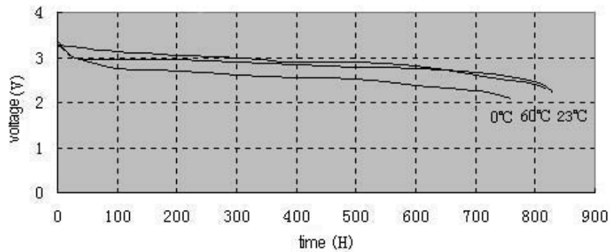
Discharge curve at various temperature (30kΩ)
