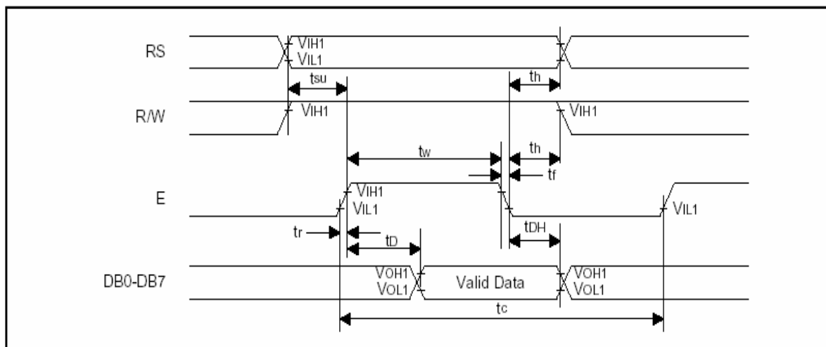
Read Mode Timing Diagram
